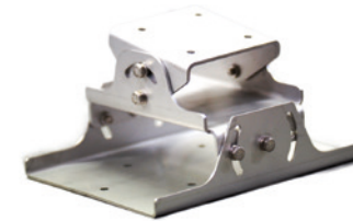
FT2 Wall mount 2-Axis Part no. 14585
